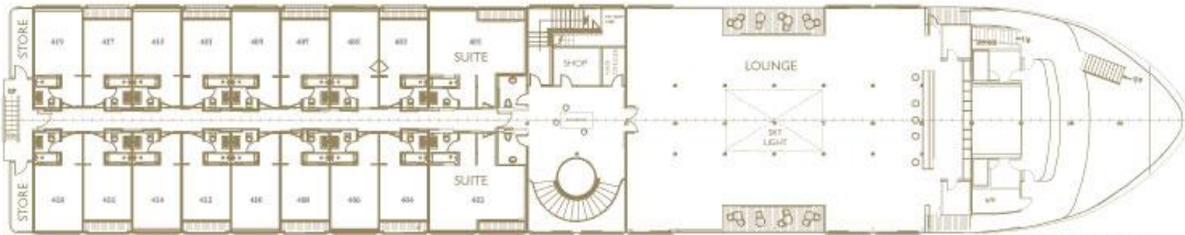
BEL AIR DECK PLAN
