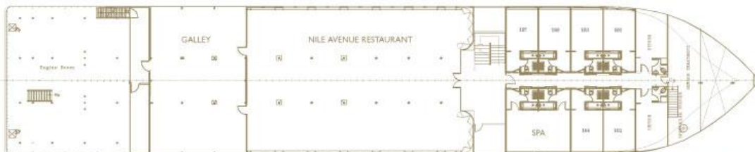
NILE DECK PLAN
