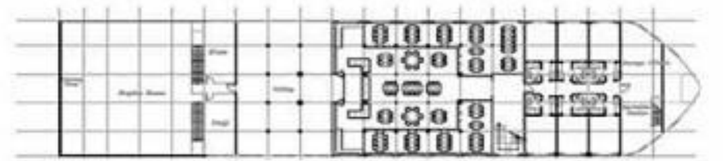
Lower Deck
