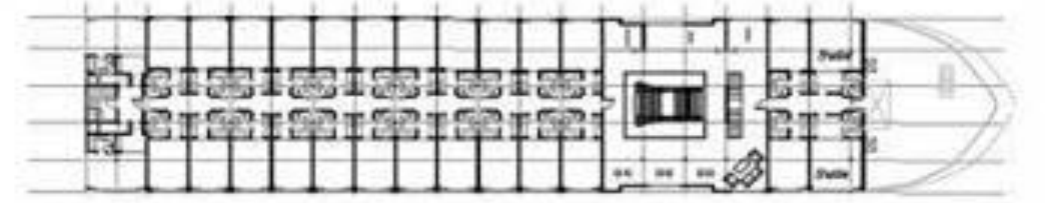
Second Deck
