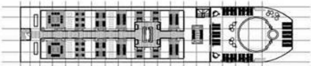
Sun Deck
