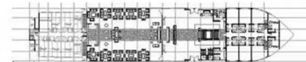
Main Deck
